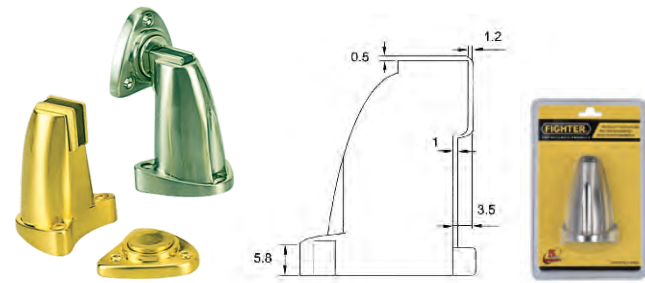
H2015 MATERIAL: Zinc Alloy
