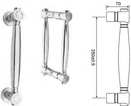
SS02016 MATERIAL: Stainless Steel or Brass
