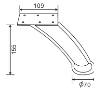
FF2020CP MATERIAL: Steel
