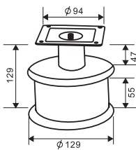
FF2003CP MATERIAL: Steel
