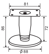
FF2010CP MATERIAL: Steel
