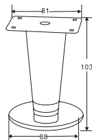
FF2007CP MATERIAL: Steel
