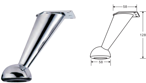
21122-128 MATERIAL: Steel
