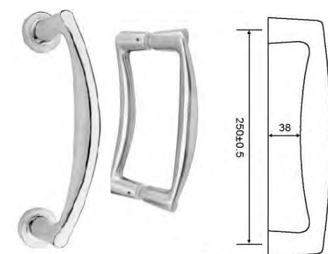
SS02017 MATERIAL: Stainless Steel or Brass
