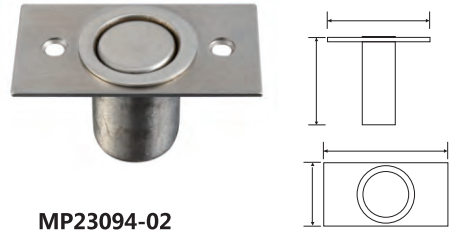
MP23094-02 Door bolt cleaner MATERIAL: Stainless Steel
