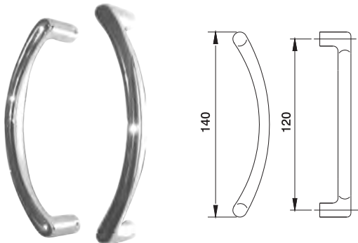
SS02022 MATERIAL: Stainless Steel or Brass
