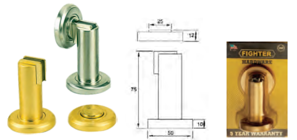
H2017 MATERIAL: Zinc Alloy
