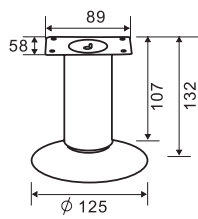
FF2002CP MATERIAL: Steel
