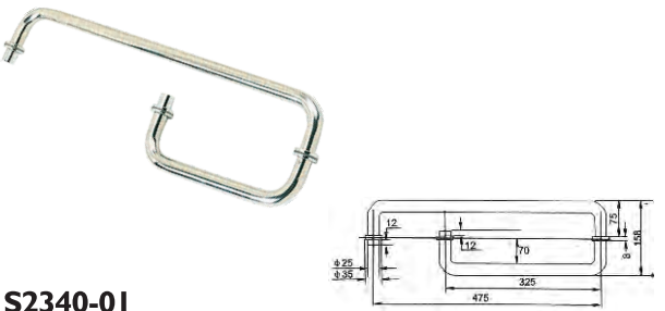
S2340-01 Bathroom glass door handle MATERIAL: Stainless Steel or Brass
