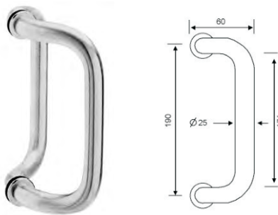
SS02019 MATERIAL: Stainless Steel or Brass
