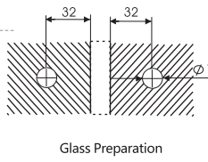
T-2604 DOOR THICKNESS: 6mm to 10mm DOOR WELGHT: 45 Kgs maximum MATERIAL: Brass
