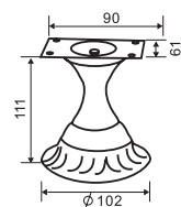
FF2011CP MATERIAL: Steel
