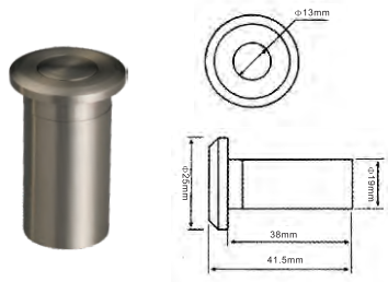
MP23094-03 Door bolt cleaner MATERIAL: Stainless Steel
