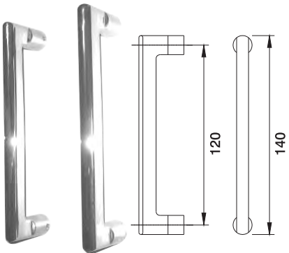
SS02018 MATERIAL: Stainless Steel or Brass
