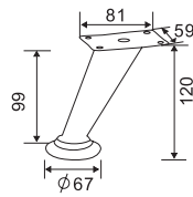
FF2017CP MATERIAL: Steel
