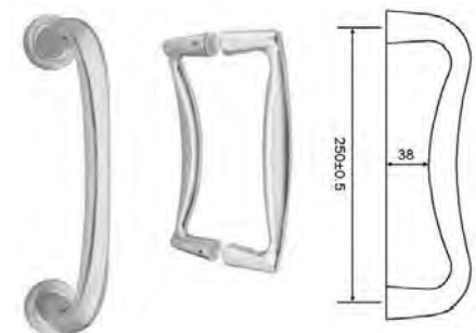
SS02013 MATERIAL: Stainless Steel or Brass
