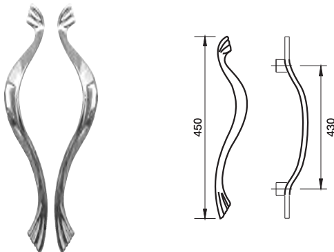
SS02024 MATERIAL: Stainless Steel or Brass
