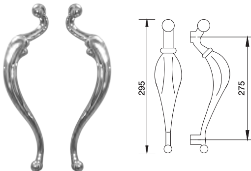
SS02023 MATERIAL: Stainless Steel or Brass
