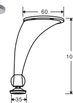
25221-100 MATERIAL: Zinc Alloy
