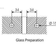
T-2606 DOOR THICKNESS: 6mm to 10mm DOOR WELGHT: 45 Kgs maximum MATERIAL: Brass
