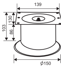
FF2004CP MATERIAL: Steel
