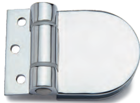
T-2603 DOOR THICKNESS: 6mm to 10mm DOOR WELGHT: 45 Kgs maximum MATERIAL: Brass
