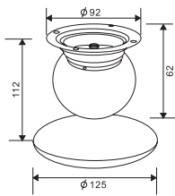
FF2001CP MATERIAL: Steel
