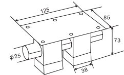
FF2025CP MATERIAL: Steel
