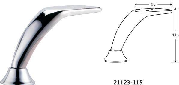
21123-115 MATERIAL: Steel
