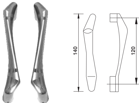
SS02025 MATERIAL: Stainless Steel or Brass
