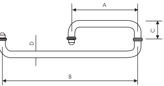
T-2760 MATERIAL: Stainless Steel or Brass
