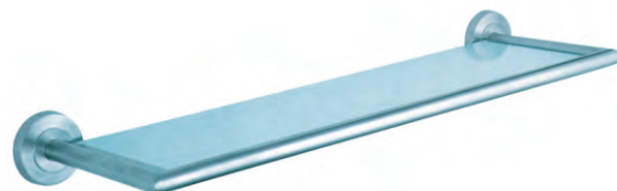
P200504 535x156x57mm MATERIAL: Stainless Steel
