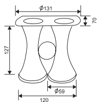
FF2005CP MATERIAL: Steel
