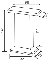
FF2015CP MATERIAL: Steel
