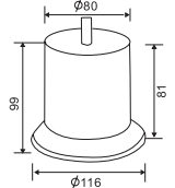
FF2014CP MATERIAL: Steel
