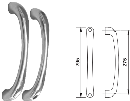
SS02021 MATERIAL: Stainless Steel or Brass
