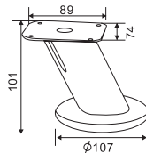
FF2013CP MATERIAL: Steel
