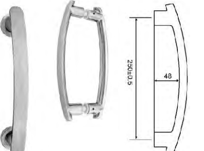
SS02014 MATERIAL: Stainless Steel or Brass
