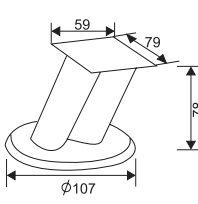
FF2006CP MATERIAL: Steel
