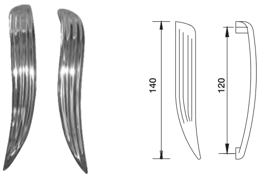
SS02026 MATERIAL: Stainless Steel or Brass
