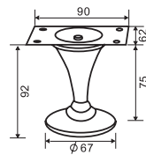
FF2009CP MATERIAL: Steel
