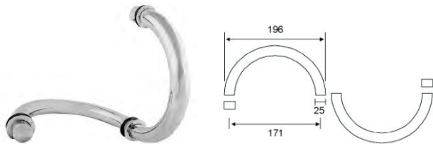
SS02020 MATERIAL: Stainless Steel or Brass
