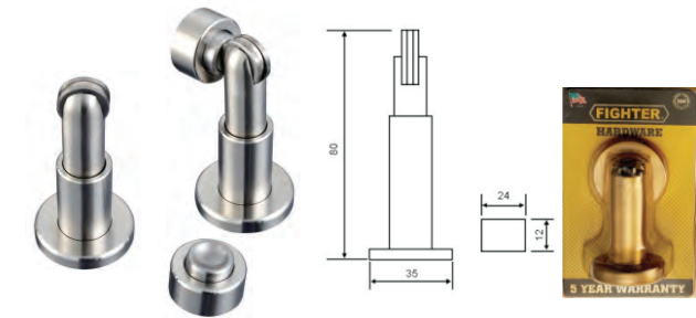
H2040 MATERIAL: 304 Stainless Steel
