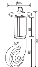
FF2027CP MATERIAL: Steel
