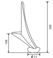
FF2019CP MATERIAL: Steel
