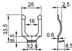
STEEL CLIP to be special order
